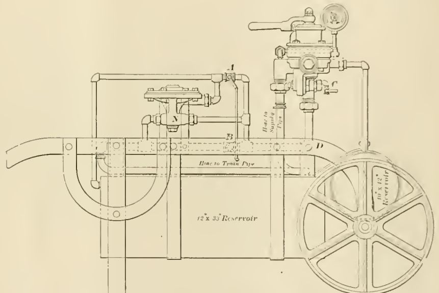
Fig. 2.—TRIPLE VALVE TESTING DEVICE MOUNTED.
